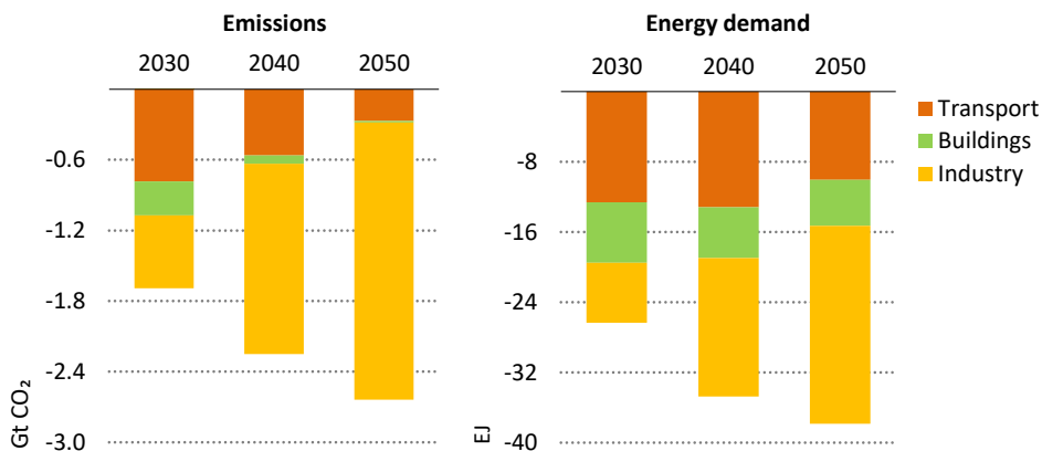
Figure 2.15 ▶ CO 2 emissions and energy demand reductions from behavioural changes and materials efficiency in the NZE
